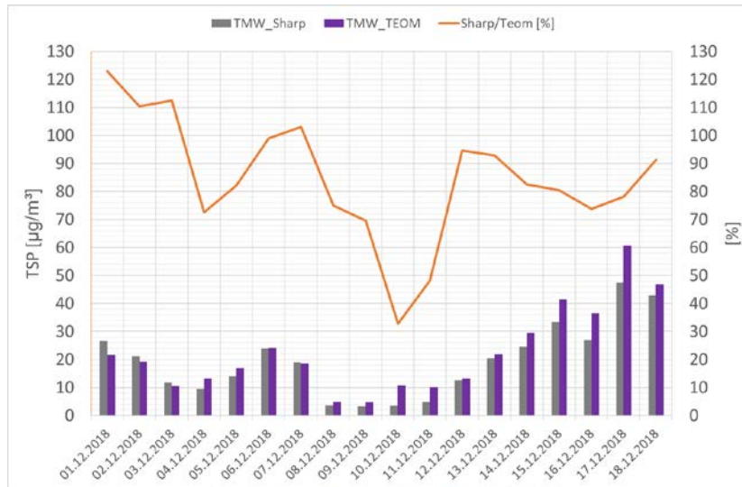
Figure 5: Comparison of TEOM and SHARP measurement systems
