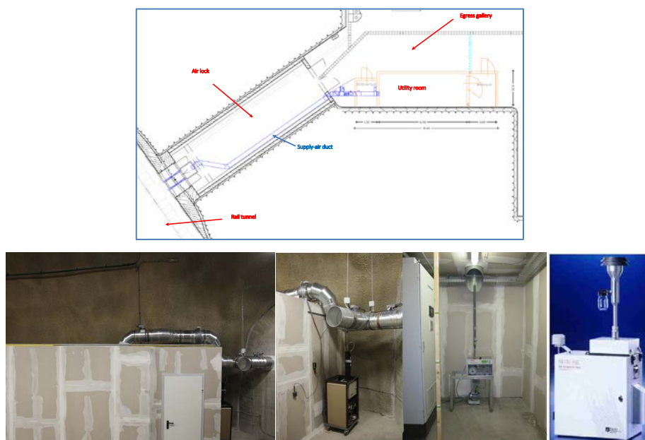
Figure 4: Test room within Unterwald evacuation tunnel – layout (above); utility room (left); PM measurement devices / TEOM, Sharp & PARTISOL (right)
