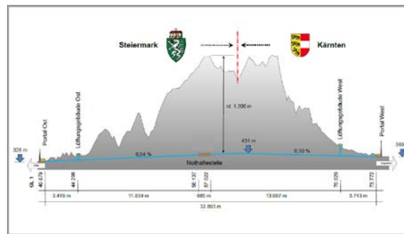
Figure 2: Longitudinal section of the Koralm Tunnel
