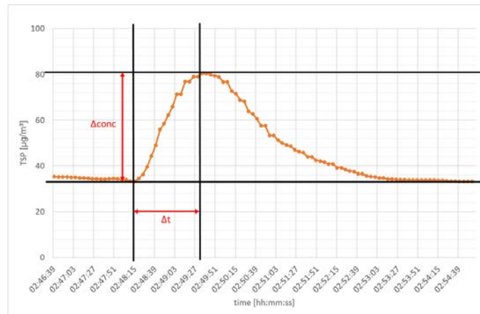
Figure 6: Concentration – time curve for a train passing the measurement location inside the tunnel
